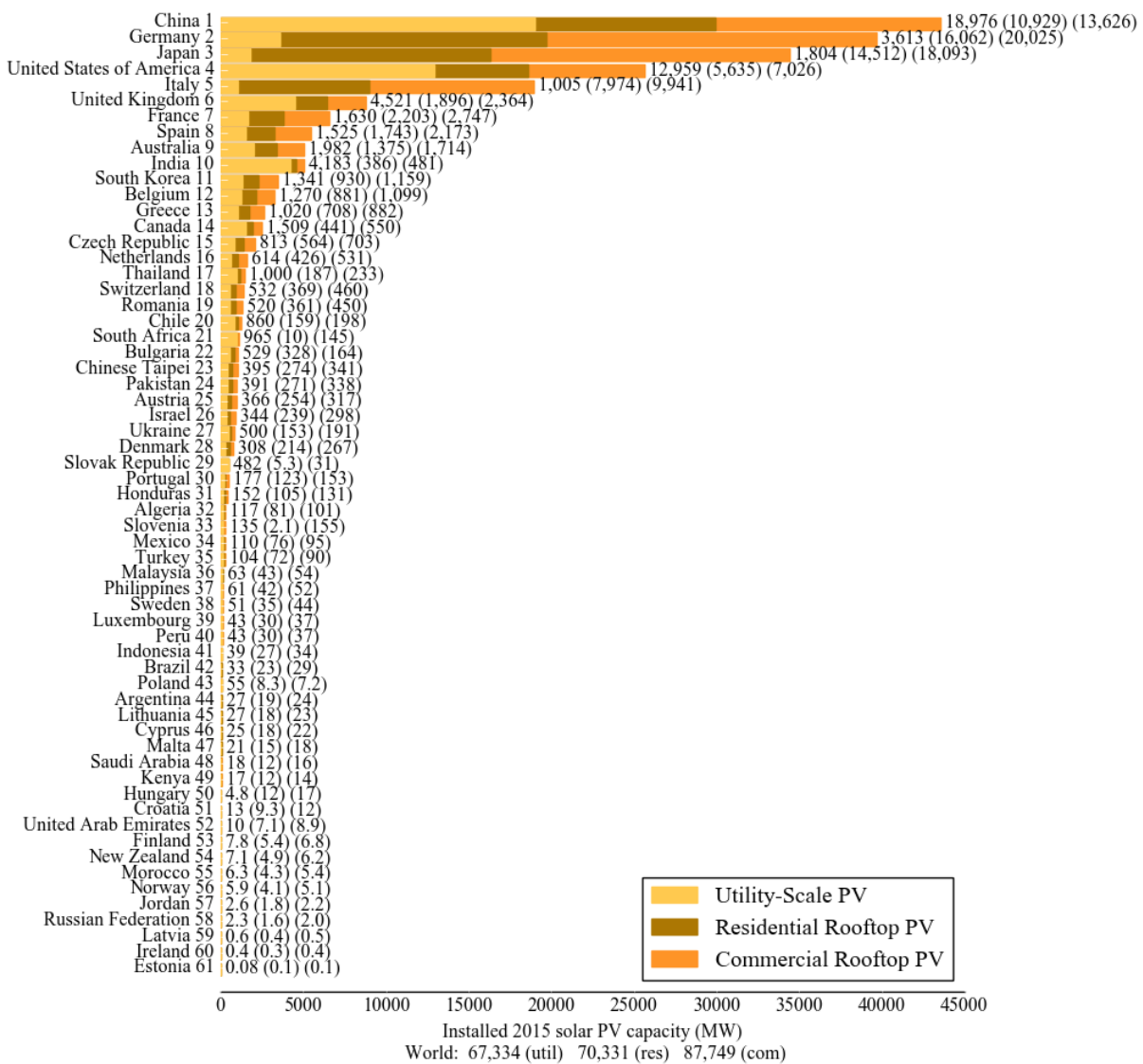
Figure S7. (a) Installed residential, commercial/government, plus utility PV by country and (b) installed CSP by country as of the end of 2015. Total PV is determined first from IEA (2016); the ratios of residential : commercial/government : utility PV for 20 European countries and global averages used on the remaining countries are from EPIA (2014). CSP by country is from CSP Plaza (2016).
