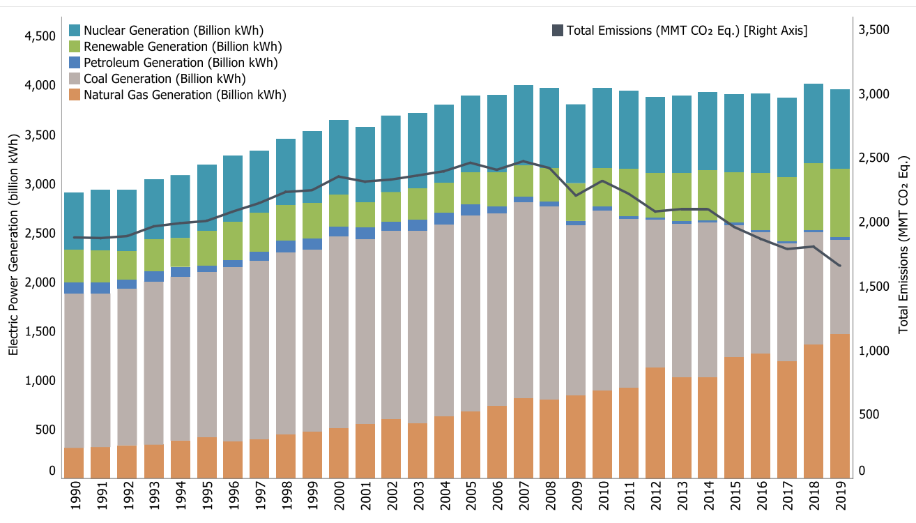
Figure ES-8: Electric Power Generation and Emissions
