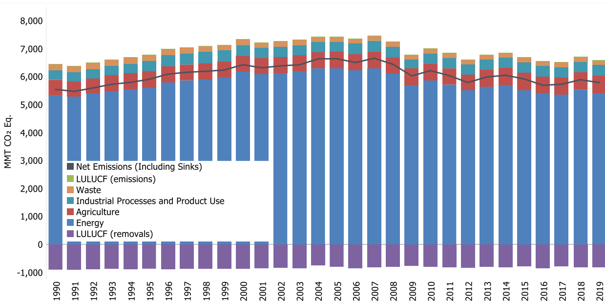
Figure ES-12: U.S. Greenhouse Gas Emissions and Sinks by Chapter/IPCC Sector
