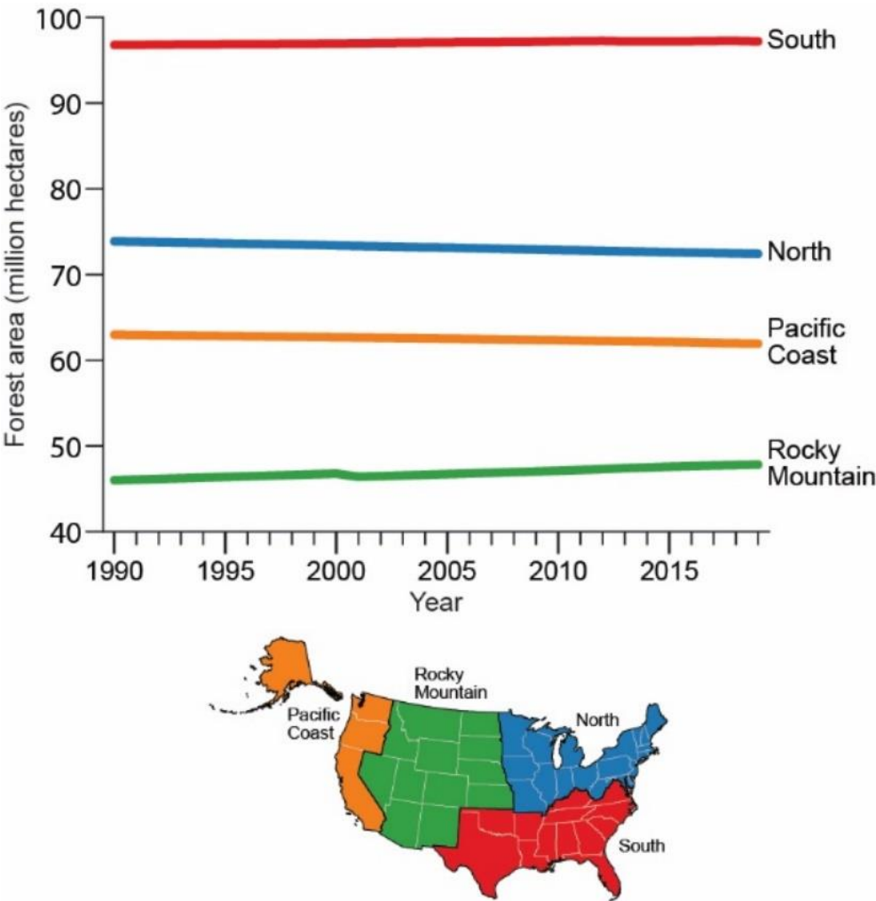
Figure 6-4: Changes in Forest Area by Region for Forest Land Remaining Forest Land in the conterminous United States and Alaska (1990-2019)
