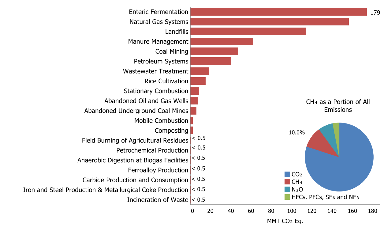
Figure ES-9: 2019 Sources of CH 4 Emissions
