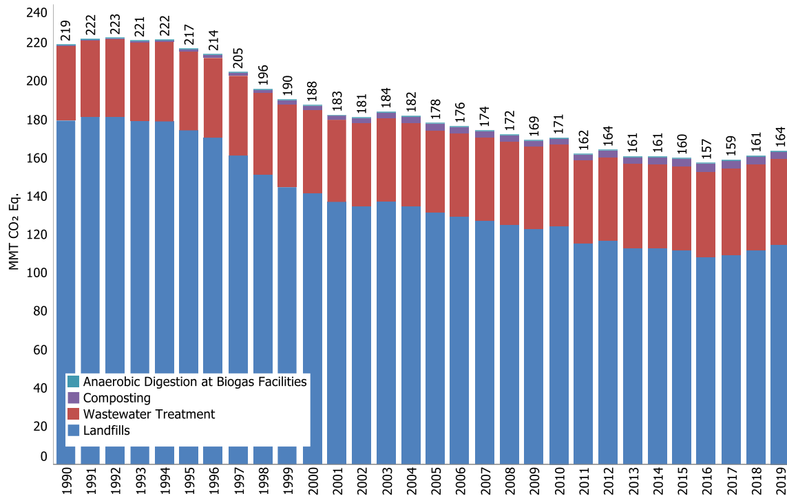
Figure 2-17: Trends in Waste Chapter Greenhouse Gas Sources
